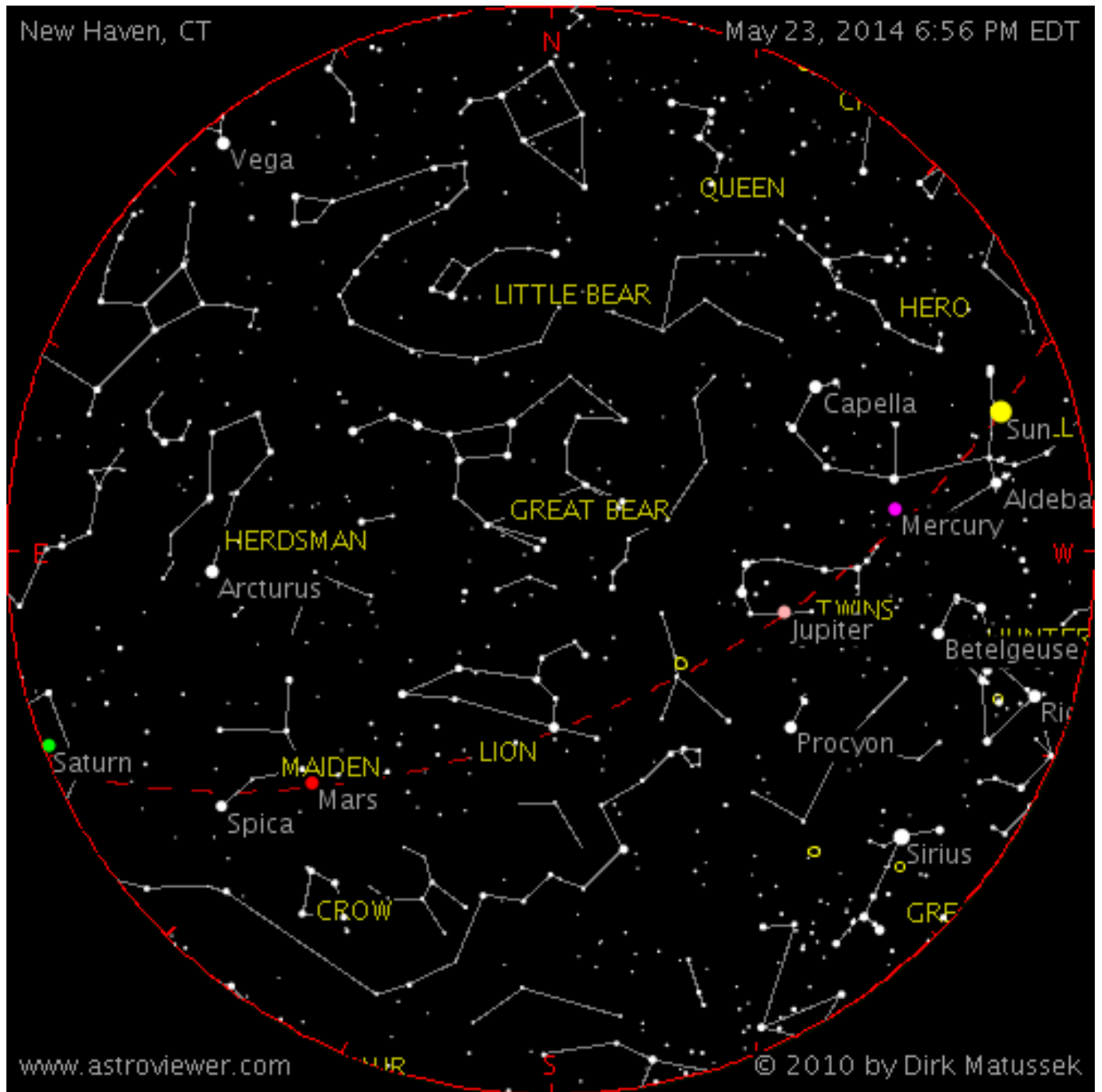
Sky map by AstroViewer
